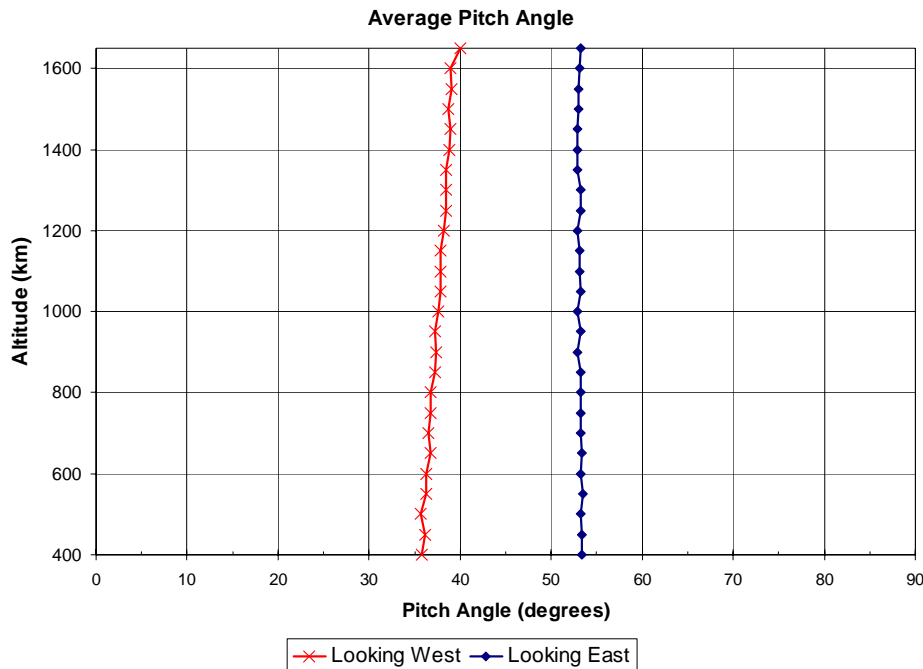
Figure 3.7: Average pitch angles of the CEASE primary look vector for east and west looking measurements in the -30^{\circ} Lat, 315^{\circ} Long stack at each altitude
