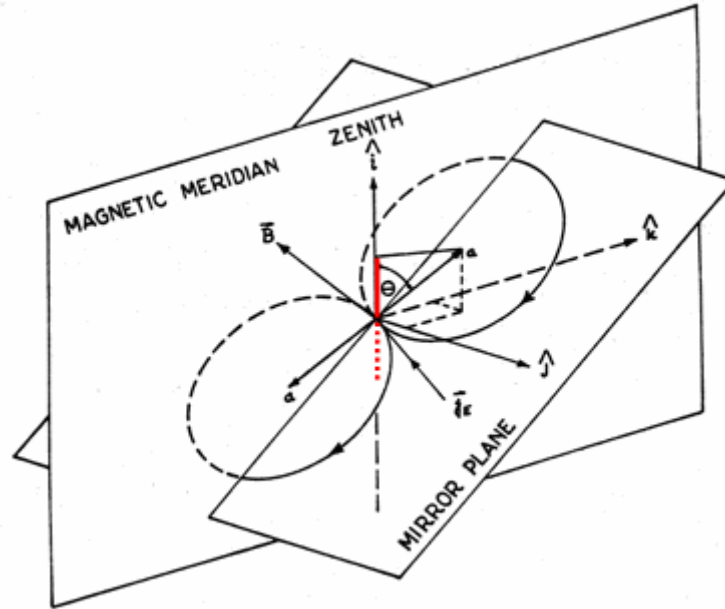
Figure A.1: Geometry showing the difference in altitude between the centers of the gyro-radii corresponding to the eastward and westward fluxes [Heckman et al., 1963]
